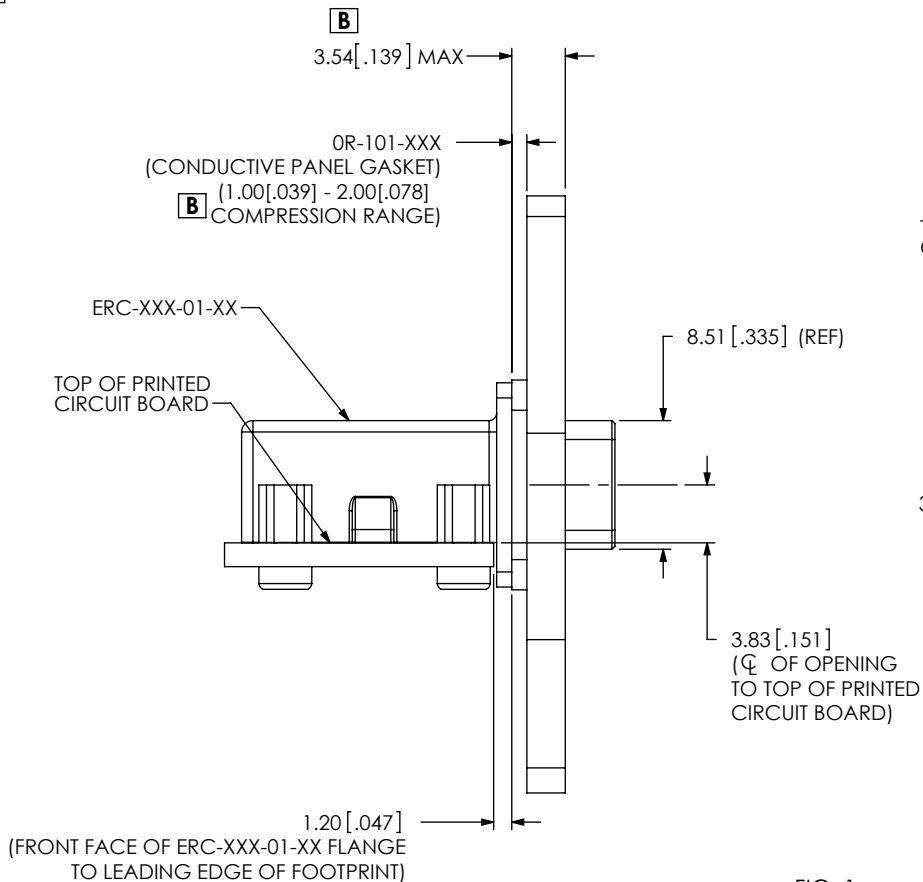
FIG. 1 (ERC-XXX-01-02 ASSEMBLED TO PANEL) (WITH GASKET)
